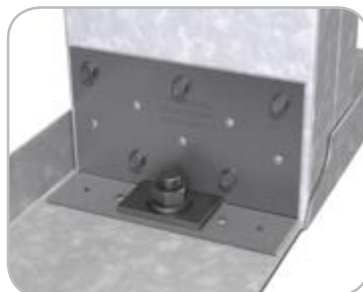
Installation with washer
